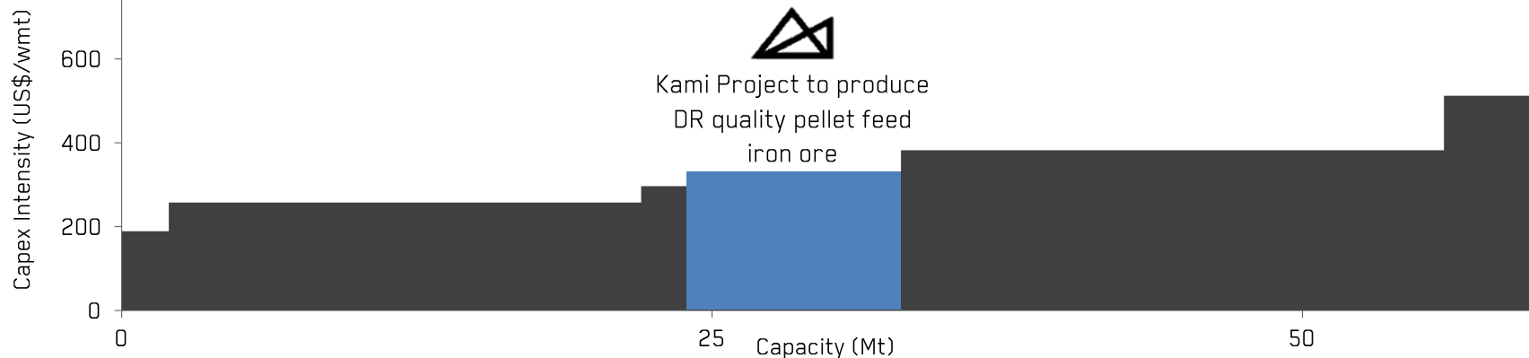
HIGH-PURITY FE GREENFIELD COMPLETED PROJECTS CAPEX INTENSITY (2014-2022) (US$/wmt)
